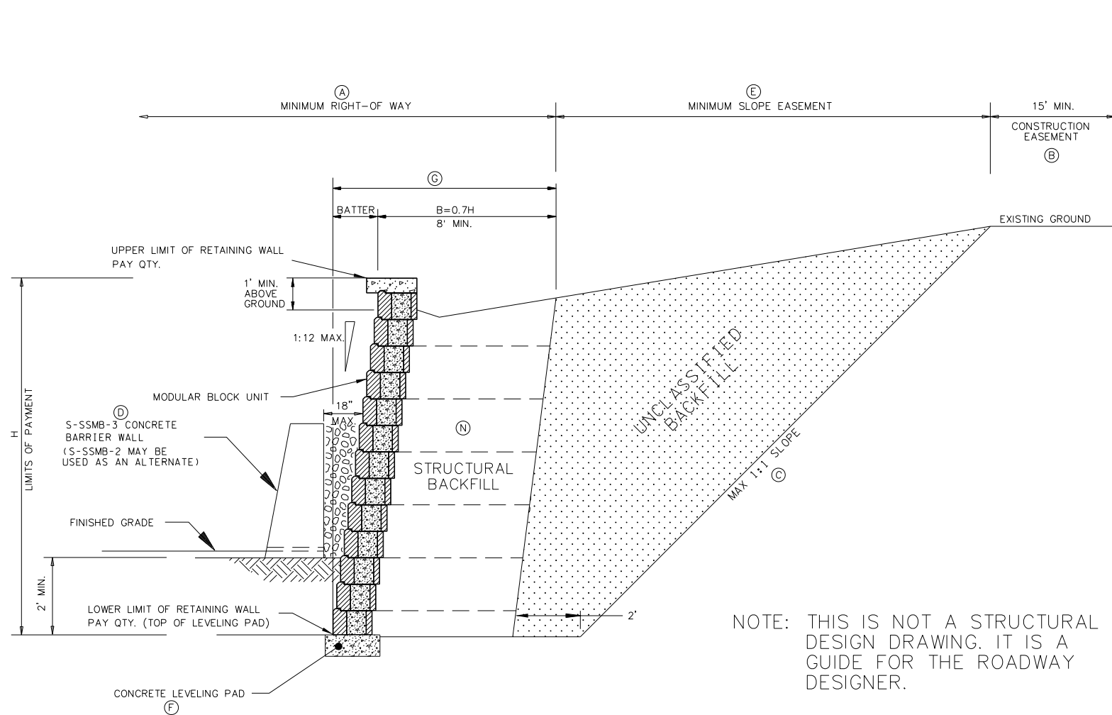
MECHANICALLY STABILIZED EARTH (MSE) WALL MODULAR BLOCK TYPICAL SECTION IN CUT (NOT RECOMMENDED IN CUT SECTIONS)
