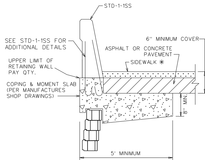
CONCRETE BARRIER ATTACHMENT DETAIL TO BE PROVIDED BY MANUFACTURE
